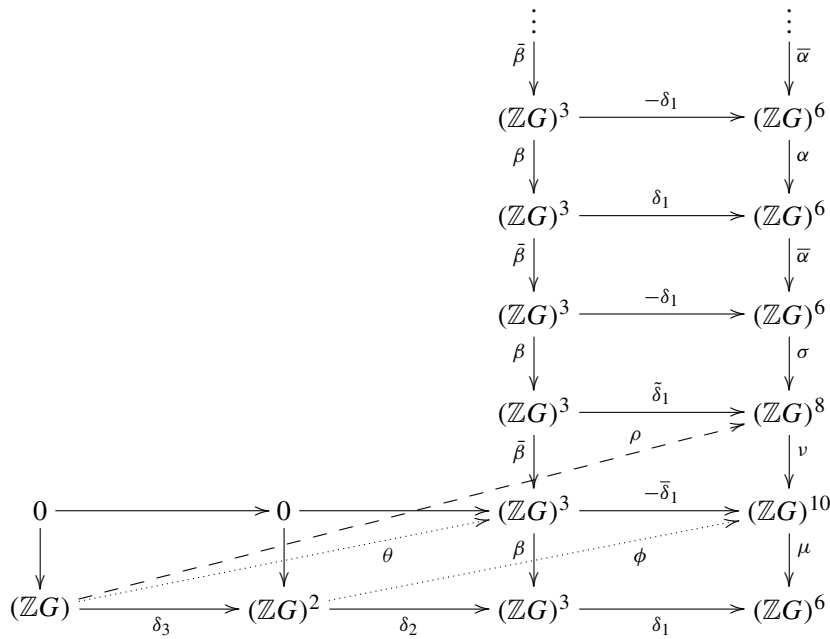
Figure 5. System of free \mathbb{Z}G -modules.
